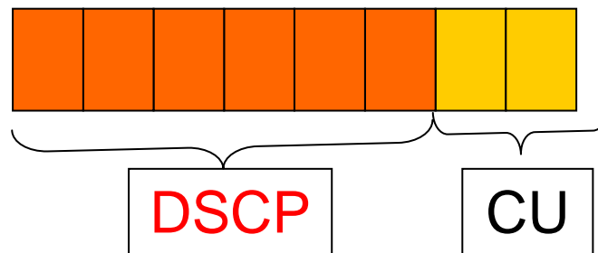
Figura 9: Formato do byte do Differentiated Service (DS) [44]
